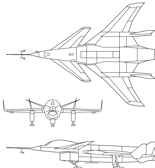
HiMat (Highly Maneuverable Aircraft Technology)
