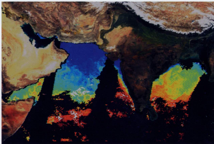
Figure 3 Photosynthetic Activity
