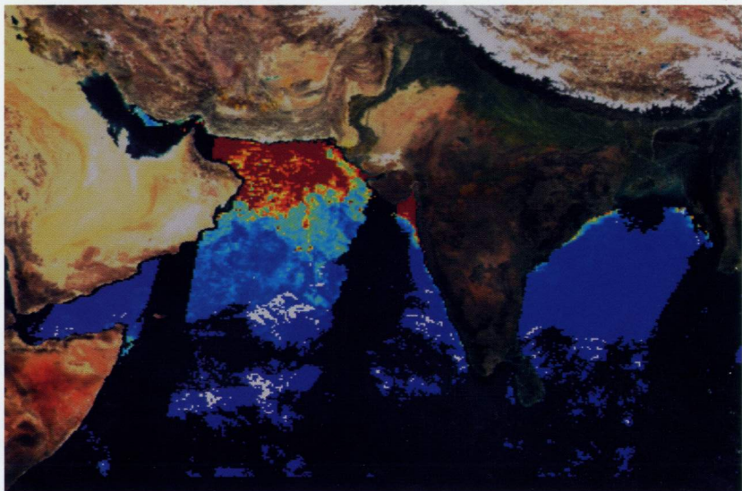
Figure 1 Chlorophyll Concentrations
