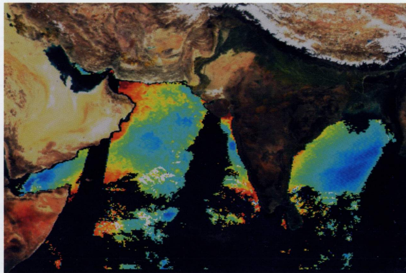
Figure 2 Chlorophyll Fluorescence
