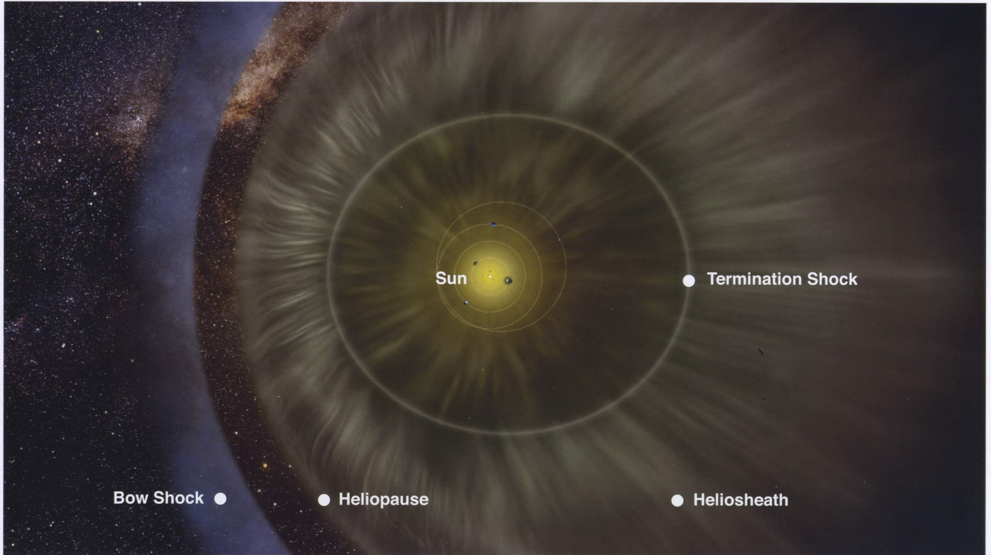
The Heliosphere
