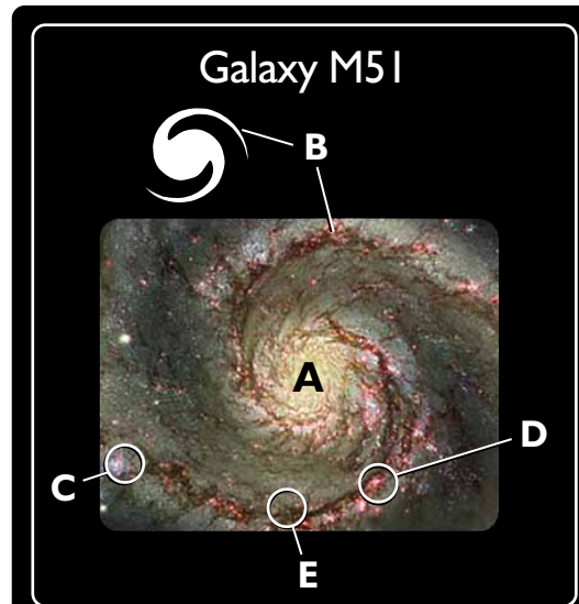
M51 spiral galaxy. Central bulge (A); spiral arm (B); clusters of young, hot stars (C); glowing hydrogen gas (D); dust clouds (E).
